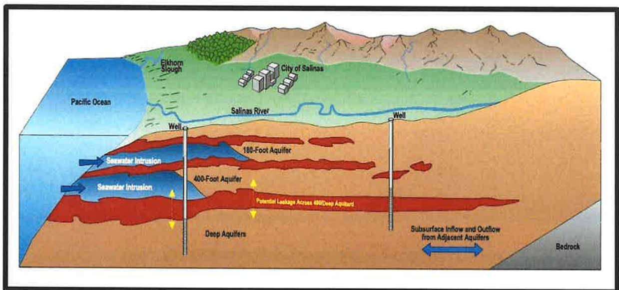
Figure 1 – Simplified profile of Salinas Valley hydrogeology
